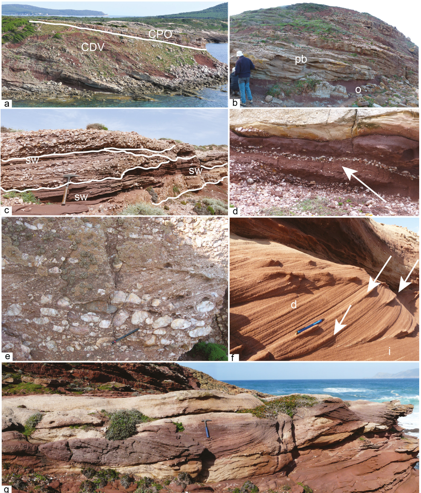
Fig. 4 - Field view of the Cala del Vino fm. and Porticciolo conglomerate, and relative lithofacies. (a) Panoramic view of southern Porticciolo gulf showing the unconformable contact between the Permian Cala del Vino (CDV) and the Triassic Porticciolo conglomerate (CPO) formations. Note the alternation of sandy fluvial bars and pelitic overbank facies in CDV deposits. (b) A fluvial point bar in the CDV (pb) overlying overbank reddish pelites (o). (c) Tightly-packed breccia/conglomerate beds with an erosive base intercalated to sand wedges (sw) in the CPO a lithofacies. (d) Palaeo-reg with in-situ strings of ventifacts (arrow), inside medium size reddish sandstones in lithofacies CPO b . (e) Clast-supported pebbly conglomerates (inclined pen for scale, showing imbrication) in CPO a lithofacies. (f) Aeolian dunes in CPO b lithofacies with dune-interdune laminations (arrows show grain flow episodes). (g) Large scale fluvial trough-cross stratification in upper part of lithofacies CPO b .
