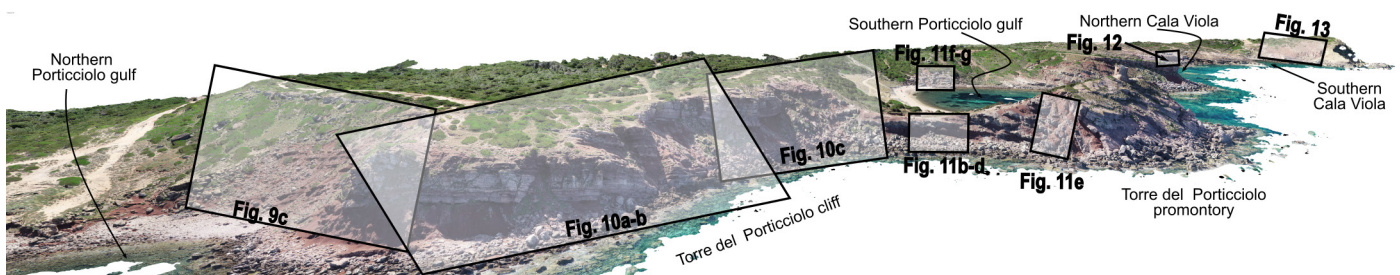
Fig. 8 - DOM of the study area from the north in which the selected outcrops are highlighted.
